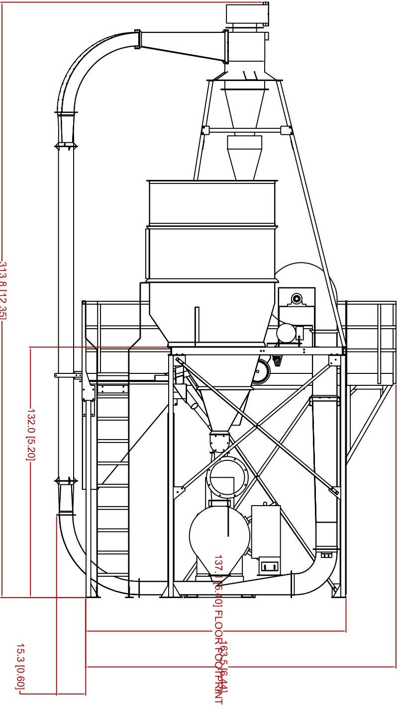
FRONT VIEW SCALE 1 / 16
