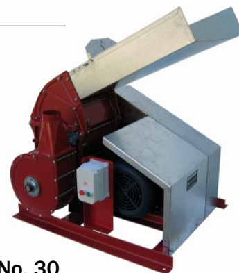
No. 30 BLOWER DISCHARGE STANDARD PACKAGE
